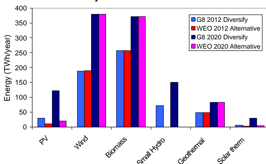
Figure SPA1. Comparison between the scenario "Diversify-Renewables" and the World Energy Outlook Alternative Power Scenario for the OECD countries
