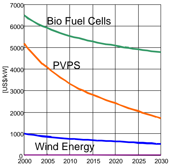
Figure SPA 2. Business as Usual Investment cost in on-grid markets
