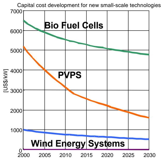
Figure SPA5. No additional on-grid. Investments cost in on-grid markets
