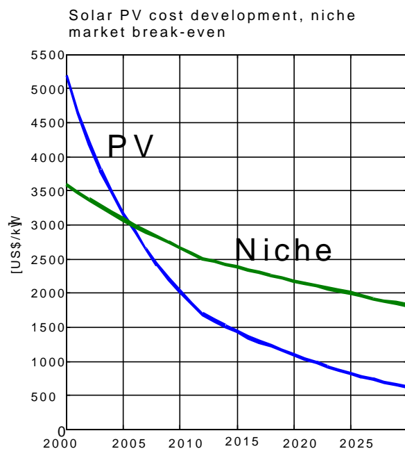
Figure SPA 4. Cost curve for PVPS and Niche Markets
